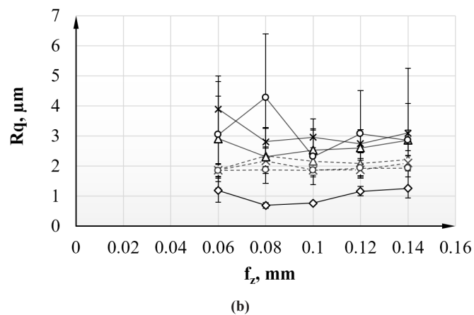
Fig. 2 Measured average roughness values (a) and root mean square values (b)
