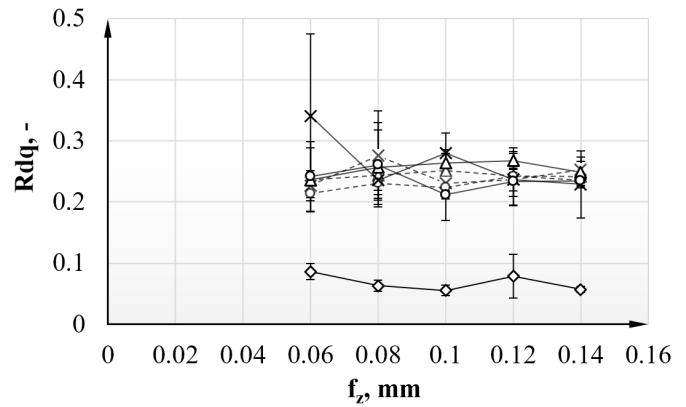
Fig. 5 The measured values of root mean square slope of the profile
