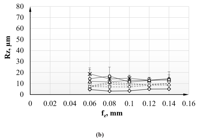
Fig. 3 Measured maximum unevenness (a) and roughness height values (b)
