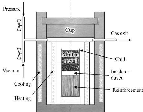
Schematic diagram of batch pressure infiltration unit [4]
