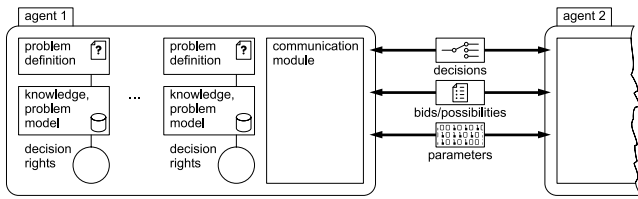
Fig. 5. Elements of conventional agent communication
