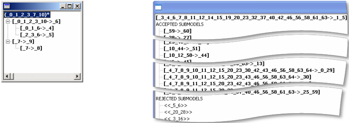
Fig. 4. Two cases of submodel decomposition. In the example to the left, the net of accepted submodels consists of five main relations (in brackets), partitioning a system containing eleven description parameters. The fourth row in the window, e.g., shows that the algorithm identified a submodel with parameters 2, 3 and 6 as inputs for the estimation of output 5. The four identified submodels have common parameters, e.g., parameter 6 is estimated by the submodel shown in the second row, but it is to be found among the input variables of the next two submodels, too. Thus, a structure of interconnected submodels can be recognized additionally to the identification of its individual parts. To the right, the result of submodel decomposition in an industrial example with a large number of system parameters is shown.
