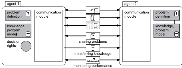
Fig. 6. Sharing an unsolved problem with other agents of the neighborhood
