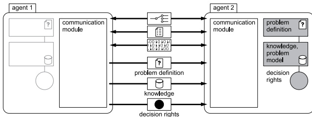
Fig. 7. Transferring knowledge and decision rights
