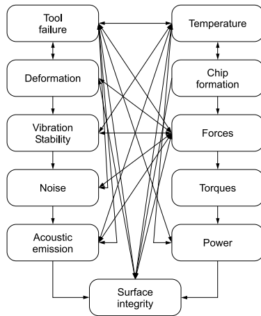
Fig. 1. A practical example for complexity: key interdependencies for a cutting process [1]. Each basic node may contain numerous parameters—the total number of variables can easily go into the hundreds for such industrial processes.
