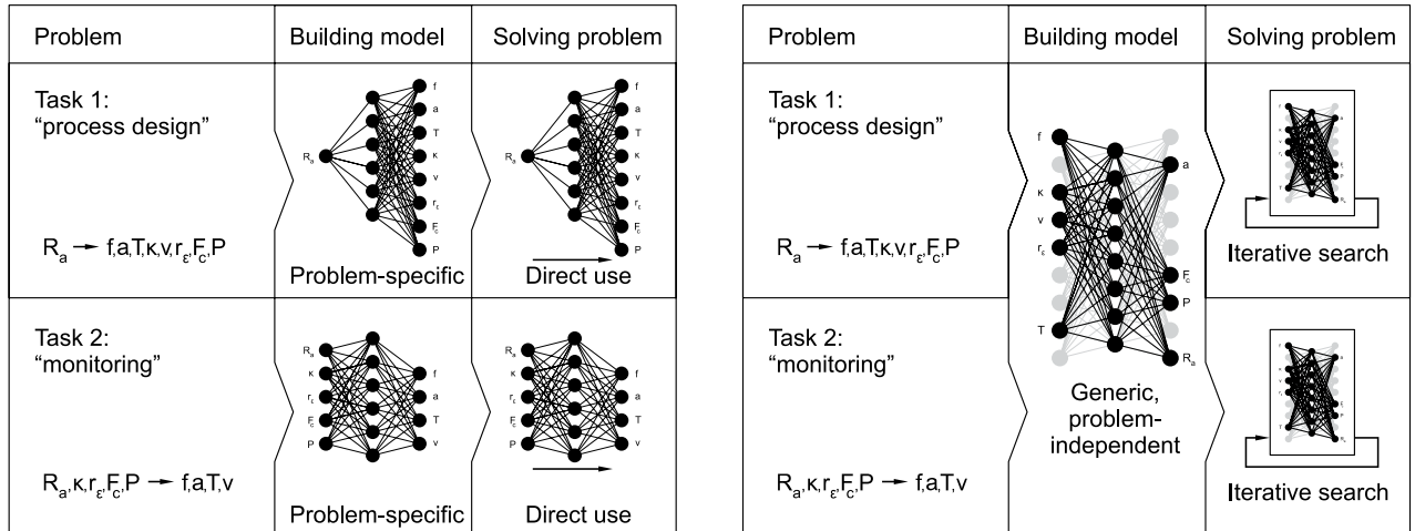
Fig. 3. Steps of problem statement, modelling and problem solving for the classical use of ANNs (left) and the task-independent generic ANN model (right)
